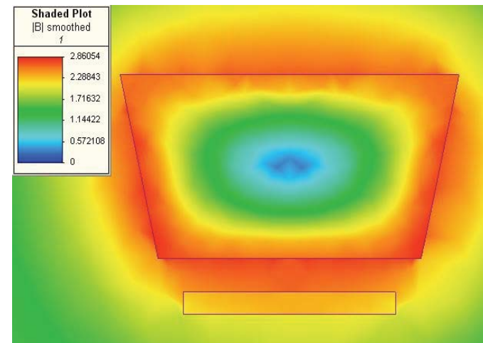
Outward taper
