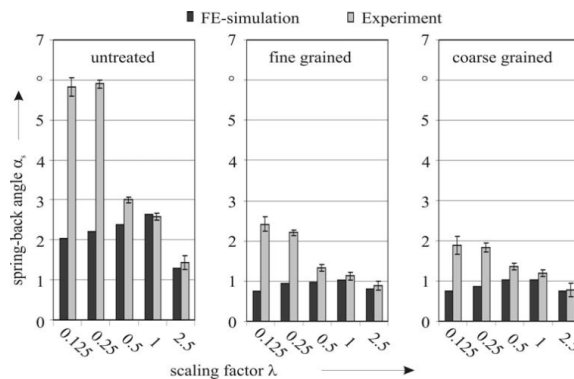
Figure 3 : Effect of miniaturization on springback angle and data scatter during bending [6]
