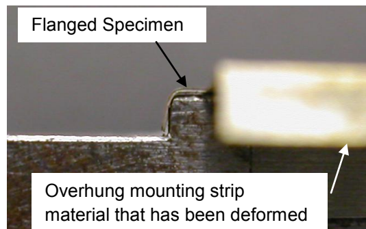
Figure 12 : Complete flanging of 0.127mm specimen
