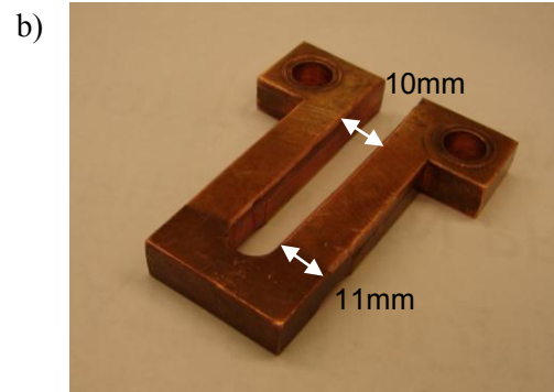
Figure 7 : Cu101 coil
