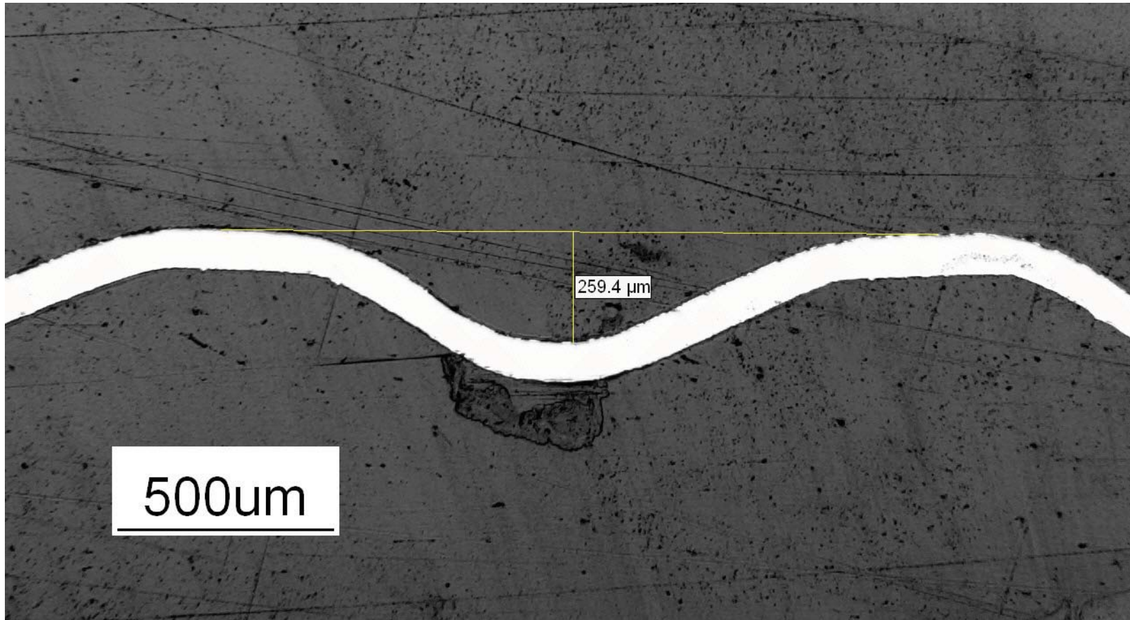
Formed part (0.1mm 439SS, 9 kJ, 260µm channel depth)
