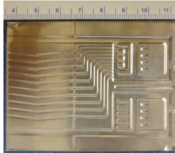
A typical formed plate (0.1mm Stainless Steel 201)
